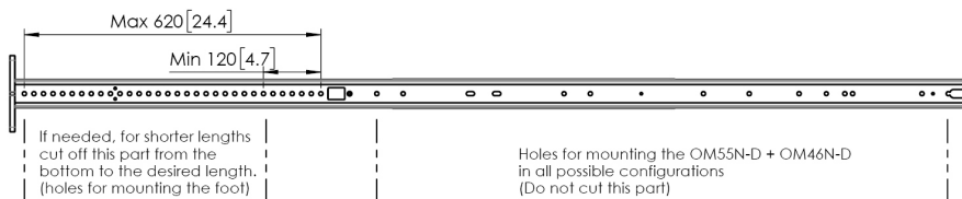
Representation of 1 profile, without covers, showing the mounting holes:
